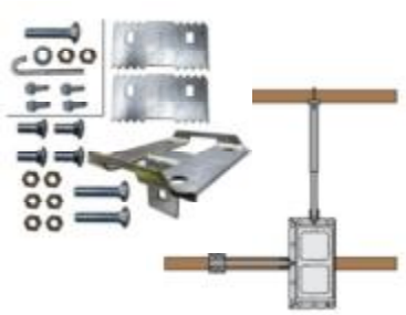
▲ 11034- Longitudinal Hardware for Standard I-Beam Frame *Required to work with either asphalt base but sold separately! For one lateral strut and one longitudinal bar.
