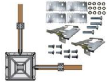
▲ 11037- Longitudinal Hardware for I-Beam Perimeter Frame *Required to work with either asphalt base but sold separately! For two longitudinal bars.
