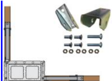
▲ 11035- Longitudinal Hardware for C-Beam Perimeter Frame *Required to work with either asphalt base but sold separately! For two longitudinal bars.
