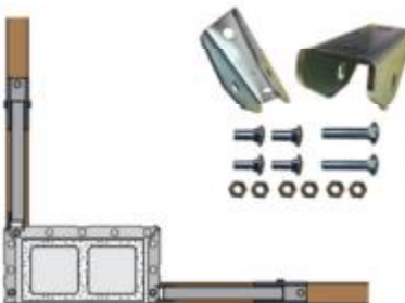
▲ 11035- Longitudinal Hardware for C-Beam Perimeter Frame
