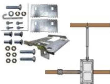
▲ 11034- Longitudinal Hardware for Standard I-Beam Frame
