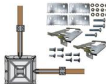
▲ 11037- Longitudinal Hardware for I-Beam Perimeter Frame
